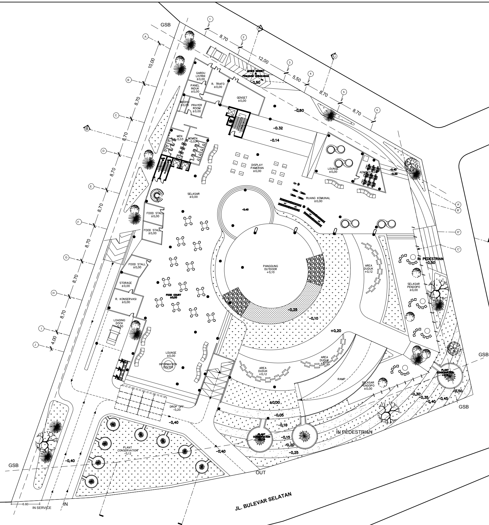
DENAH LANTAI DASAR SKALA 1:500
