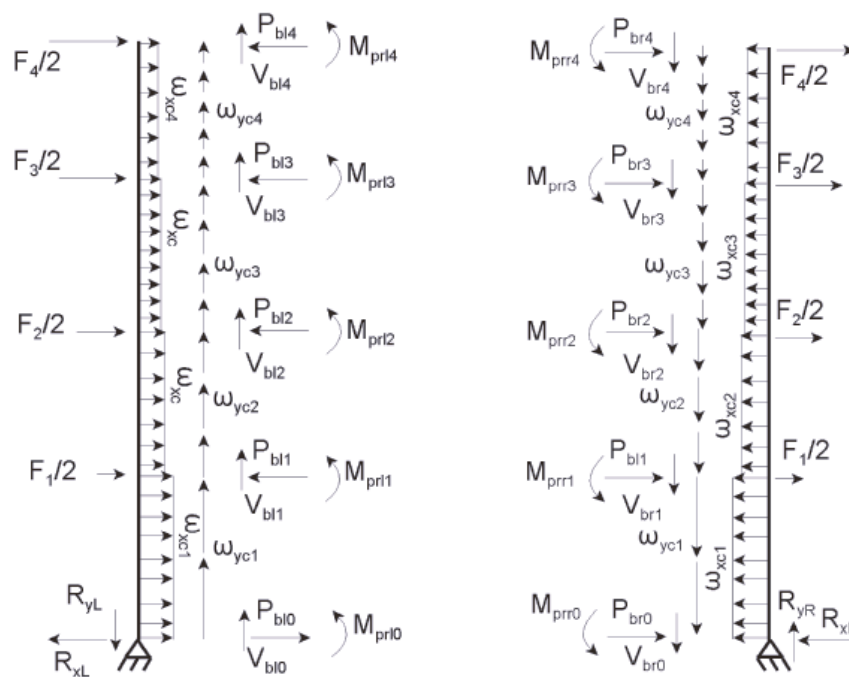
Gambar 16. Diagram free-body VBE (ANSI/AISC, 2010b)
