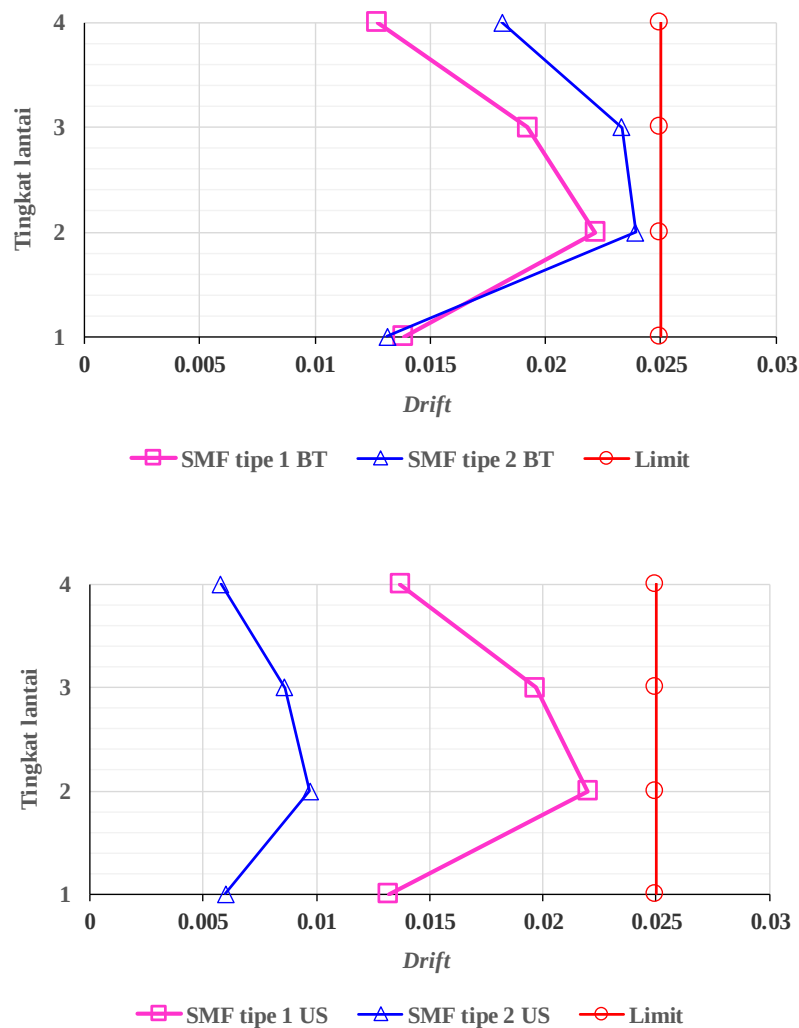
Gambar 5. Storey drift sistem SMF
