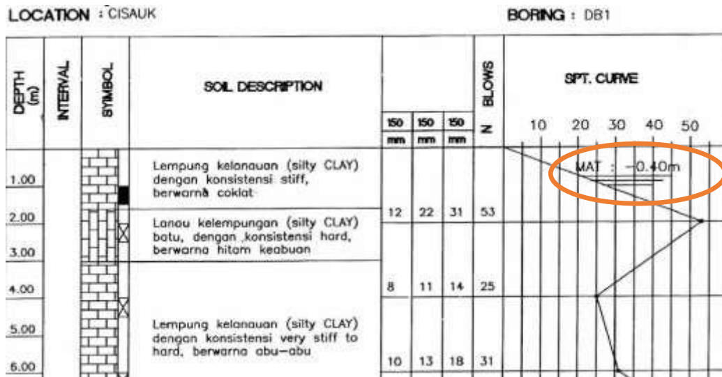
Gambar 4. Hasil boring log
