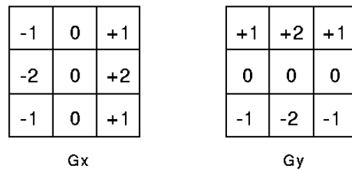
Gambar 1. Sobel operator
