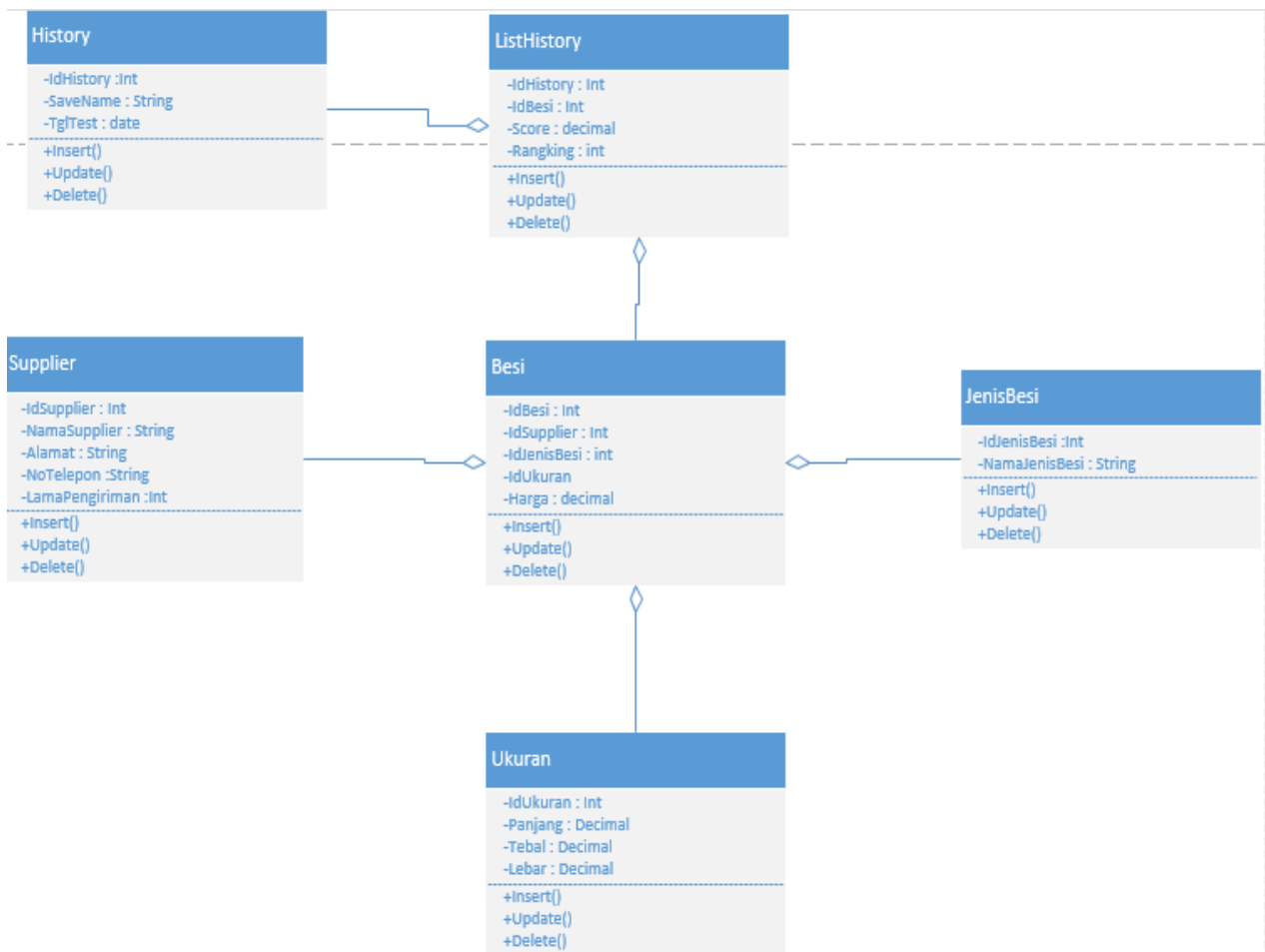
Gambar 4. Class Diagram
