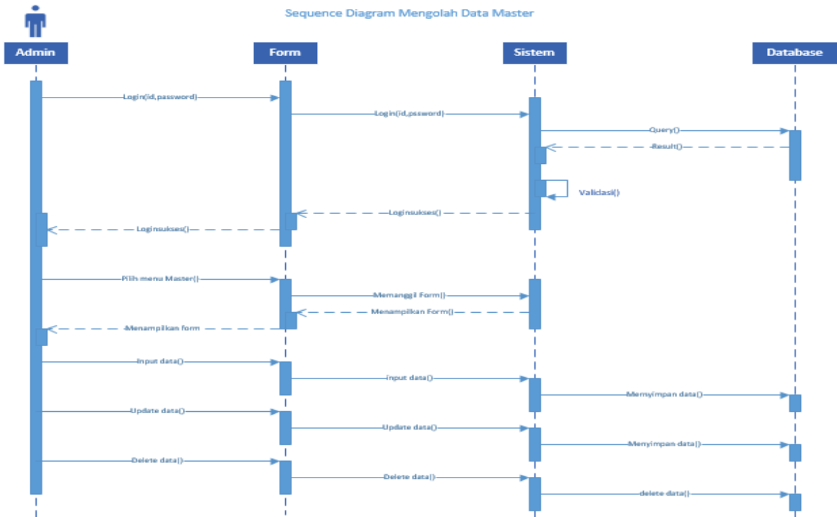
Gambar 5. Sequence Diagram
