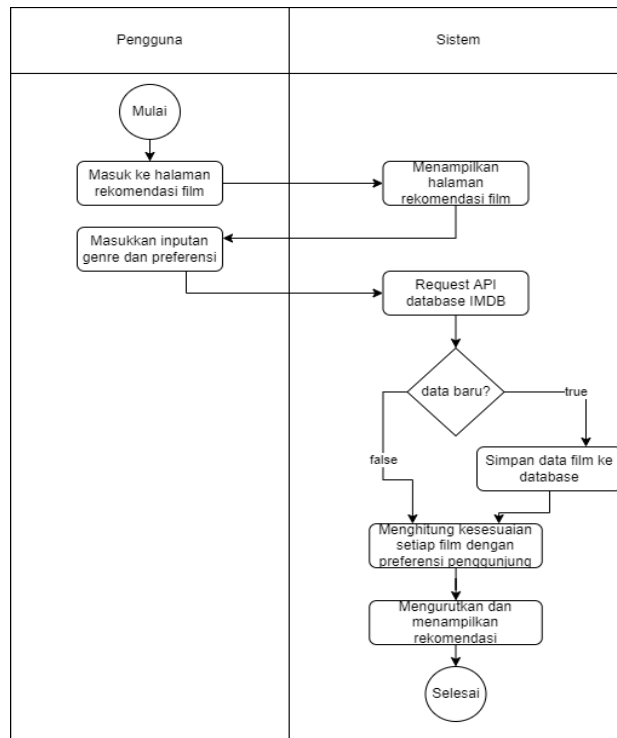
Gambar 2 Activity Diagram Sistem Rekomendasi Film
