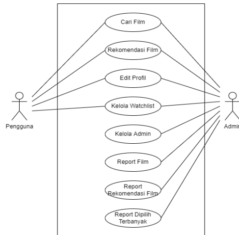
Gambar 1 Use Case Diagram Sistem Rekomendasi Film
