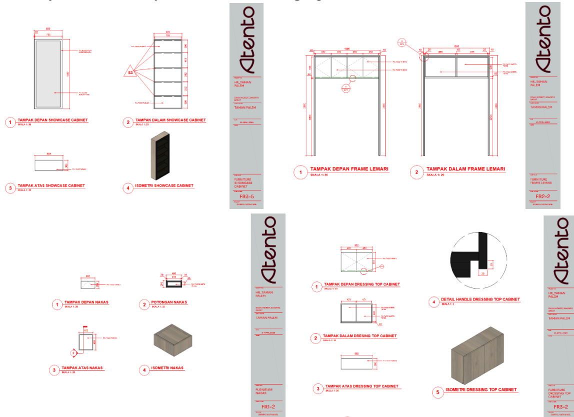
Gambar kerja cabinet kaca, frame lemari, dressing top cabinet, nakas
